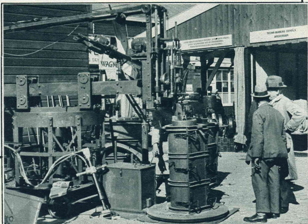
Betonstampmachine.
